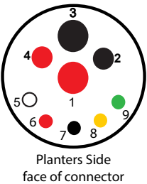
ISOBUS Connection A
