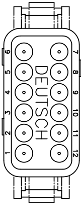
WIRE SIDE VIEW
