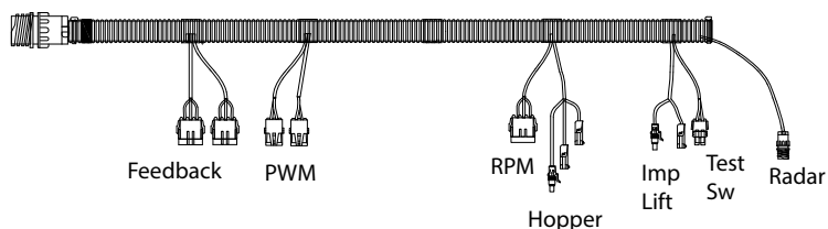
Harness PDC 46798-0162
